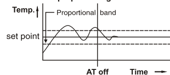
PID - time proportioning with auto reset & rate
